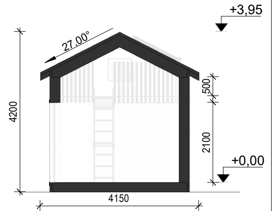
Section 1-1
