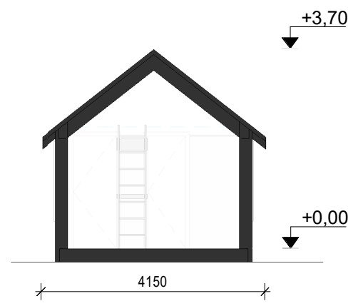
Section 1-1
