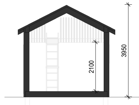
Section 1-1
