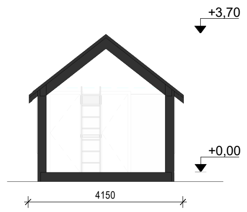
Section 1-1
